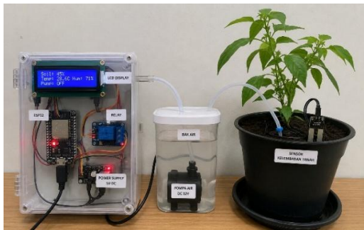
Gambar 6. Implementasi Prototype Smart Irrigation System
