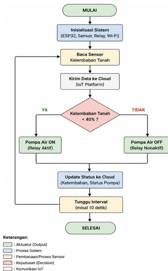
Gambar 4. Flowchart Sistem Smart Irrigation
