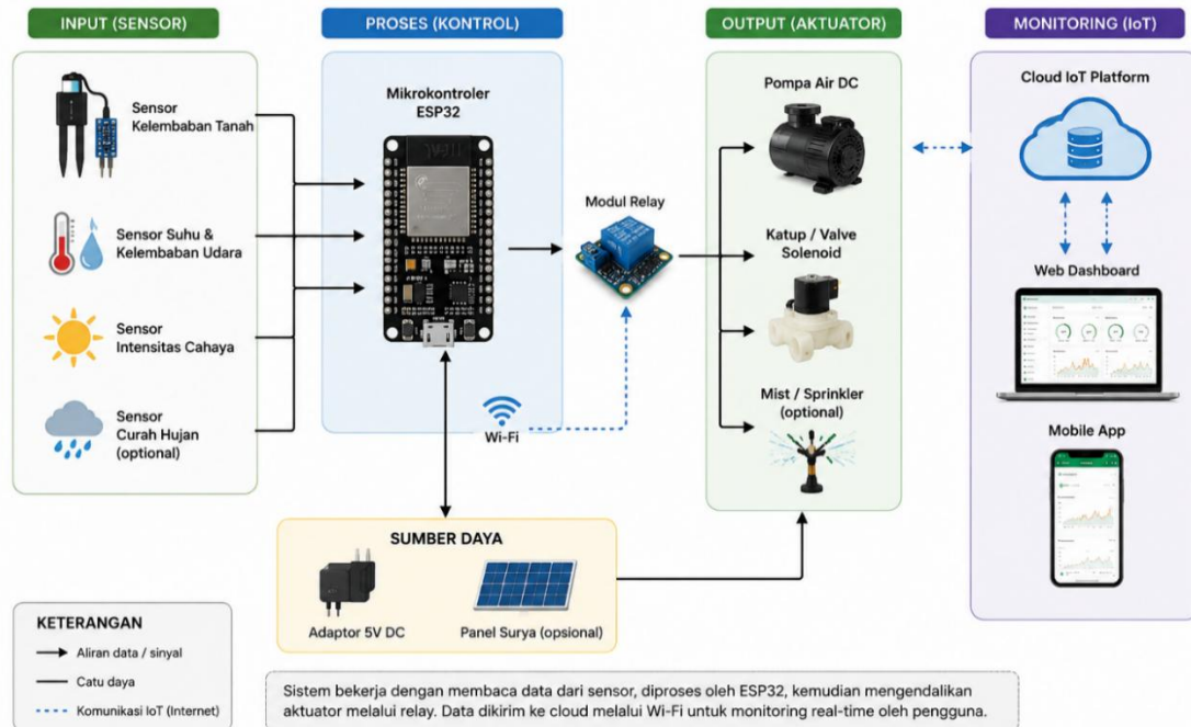
Gambar 3. Arsitektur Smart Irrigation System Berbasis IoT
